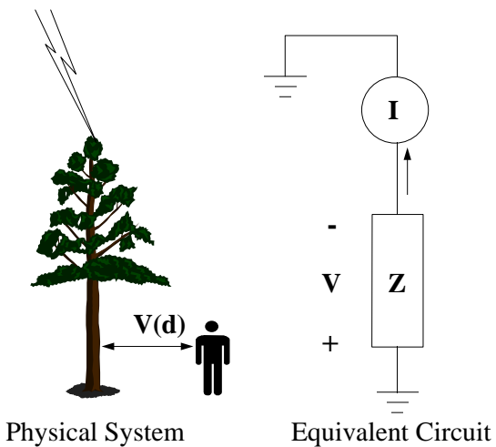
Figure 5 - Flashover Model.
